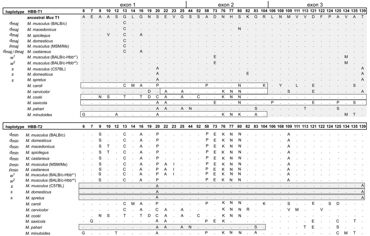
FIG. 5.—Alignment of HBB-T1 and HBB-T2 amino acid sequences from 12 Mus species showing sites that are variable in one or both paralogs. The Hbb s and Hbb p haplotypes recovered from Mus musculus are not shown as they are identical to the sequences found in the C57BL ( Hbb s ) and MSM/Ms ( Hbb p ) strains. Representative sequences are displayed for the HBB genes of M. castaneus , M. cookii , M. domesticus , and M. saxicola . HBB-T1 sequences are shown in gray and HBB-T2 sequences are shown in white. Identified gene conversion tracts are shown in boxes.
