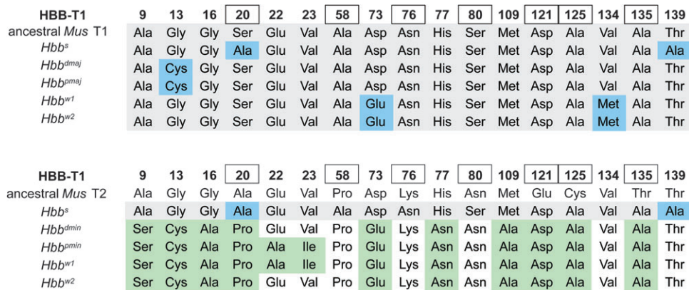
FIG. 6.—Alignment of variable amino acid sites in the HBB-T1 and HBB-T2 genes from five different haplotype backgrounds. HBB-T1 sequences are shown in gray and HBB-T2 sequences are shown in white. The Hbb s allele at HBB-T2 is shown in gray, which reflects its ectopic origin via T1 → T2 gene conversion. Substitutions that distinguish the inferred ancestral sequences of Mus HBB-T1 and HBB-T2 are denoted by boxes. Derived amino acids in HBB-T1 and HBB-T2 are shown in blue and green, respectively.
