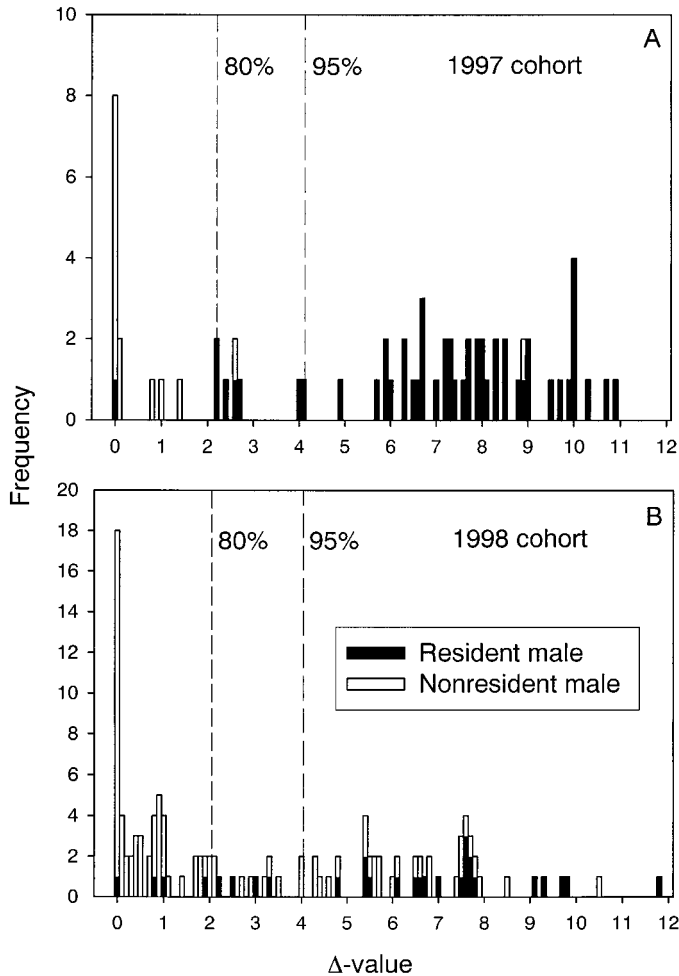
FIG. 1. Distribution of \Delta -values of most likely candidate males in the (A) 1997 and (B) 1998 offspring cohorts. Dotted lines denote critical \Delta -values for paternity assignment at 80% and 95% confidence levels. Resident males are adult males that held territories within the natal colony of a particular offspring at the time of parturition.
